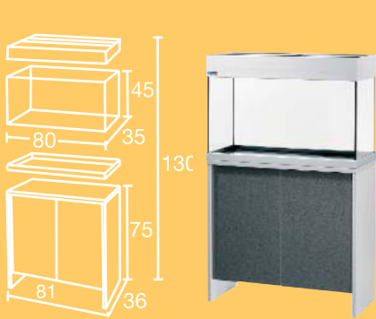
scubaline Total dimensions W x D x H cm 81 x 36 x 130
